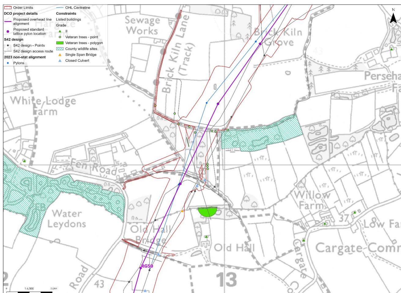
Figure 4.4 Tas Valley overhead line and construction access alignments
